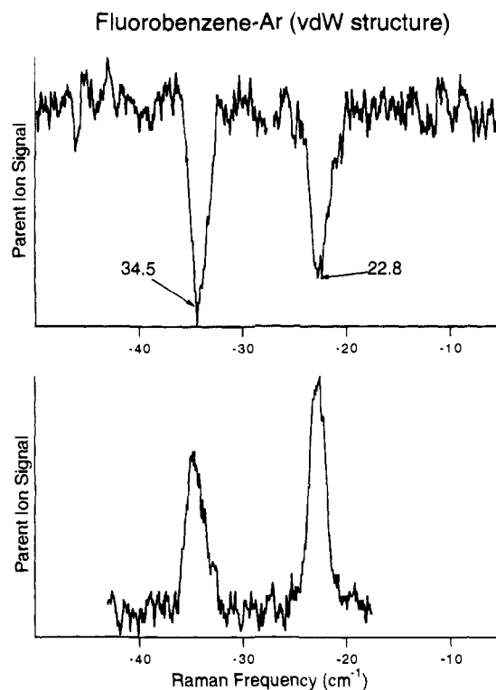
Figure 10. (Top) Mass-selective ILSRS spectrum of fluorobenzene–Ar taken in the intermolecular vibration region. To obtain these results \omega_3 was tuned to the S_1 \leftarrow S_0 0_0^0 band of the complex. (Bottom) Mass-selective IGSRs spectrum of fluorobenzene–Ar in the intermolecular vibration region. To obtain these results \omega_3 was tuned slightly to the red of the 0_0^0 band.
