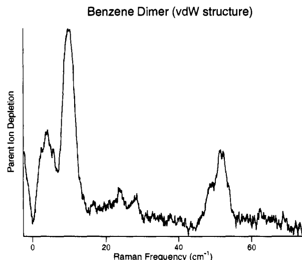
Figure 5. Mass-selective ILSRS spectrum of the fully protonated benzene dimer in the low-frequency (intermolecular vibrational) region. To obtain this spectrum \omega_3 was set to the S_1 \leftarrow S_0 0_0^0 band of the species.
